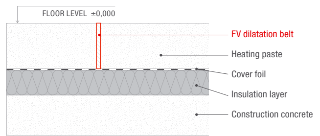
Figure 4: Heating paste dilatation joint
